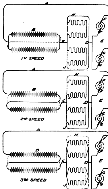
FIG. 302.—Diagram of the Circuit-Changing Arrangements of a Typical Electrical Vehicle. The full lines in these plans indicate the closed or active, circuits; the dotted lines the open, or inactive, circuits. As may be readily understood, the whole scheme of circuit-changing depends on employing several different circuit connections between battery and motor, which may be opened and closed, as desired. Here A and C are the lead wires between battery, B , and motor brushes, F F and G G , and the field-windings, H and J , and wire, D .
